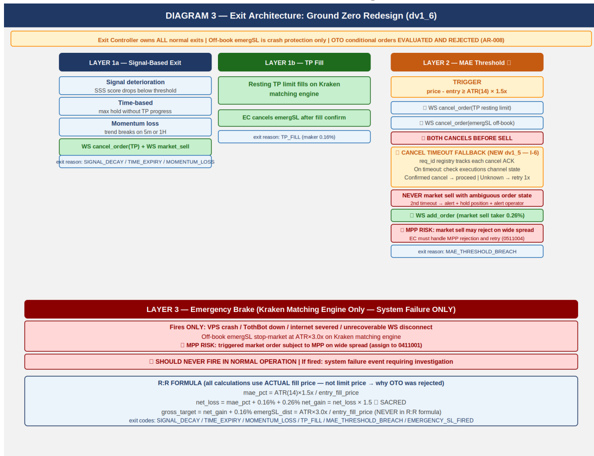
DIAGRAM 3 — Exit Architecture: Ground Zero Redesign (dv1_6)
