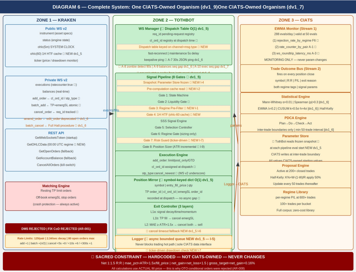
DIAGRAM 6 — Complete System: One CIATS-Owned Organism (dv1_9)
